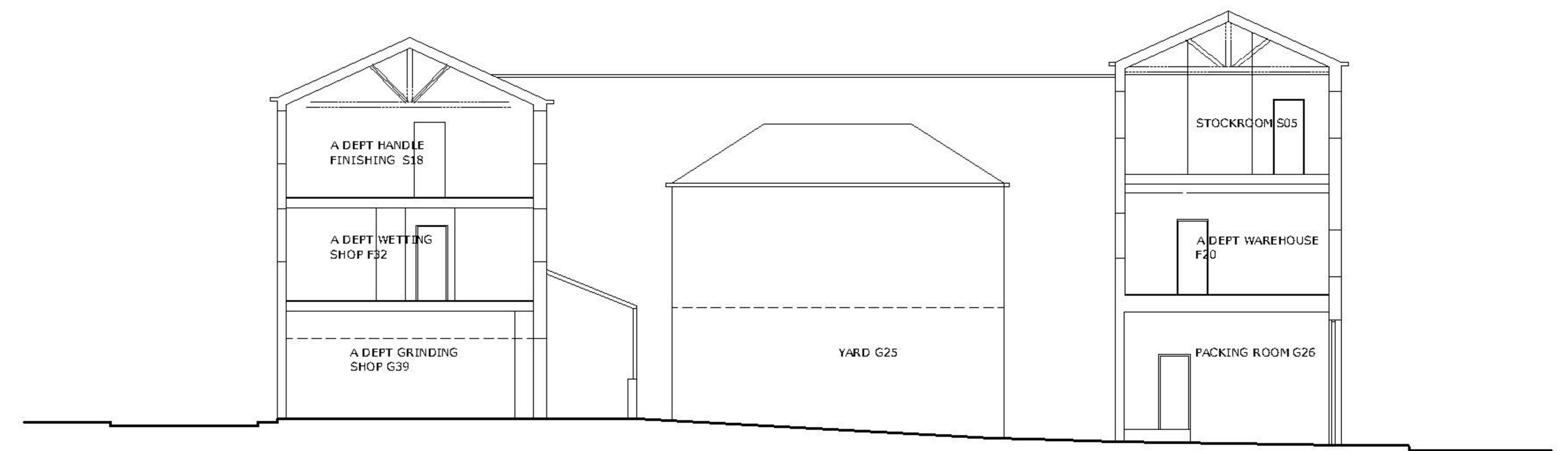
SECTION B-B
